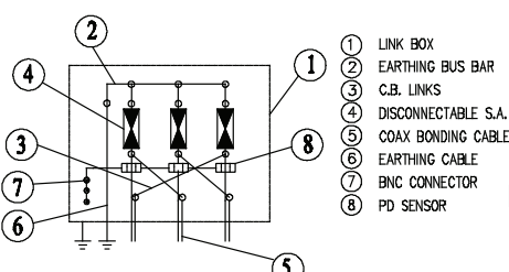
CT/BIC COUPLER TERMINATION BOX
