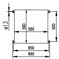
CT/BIC COUPLER TERMINATION BOX
